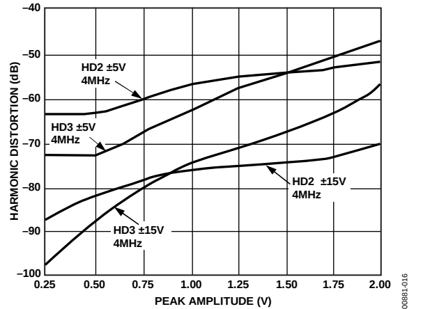
Figure 16. Harmonic Distortion vs. Peak Amplitude, Frequency = 4 MHz
