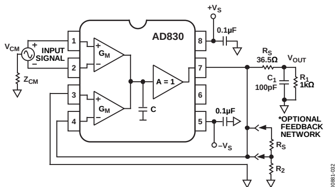
Figure 32. Circuit for Driving Large Capacitive Loads
