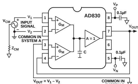
Figure 38. Differential Line Receiver
