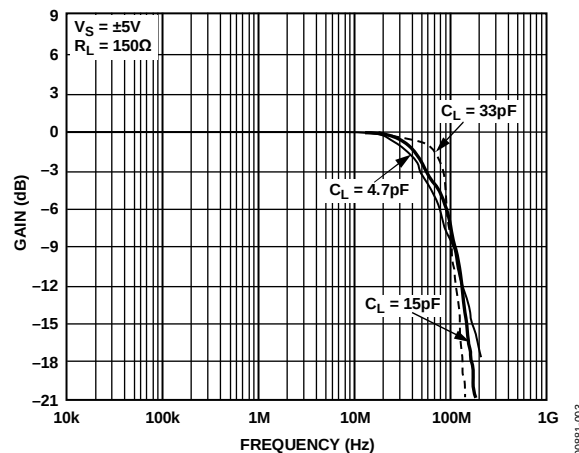
Figure 3. Closed-Loop Gain vs. Frequency, Gain = +1
