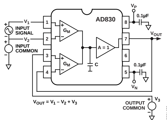
Figure 39. Differential Amplification with Level Shifting
