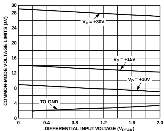
Figure 36. Input Common-Mode Range for Single Supply
