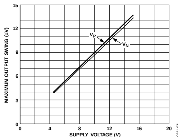
Figure 31. Maximum Output Swing vs. Supply
