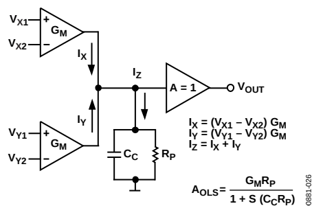
Figure 26. Topology Diagram
