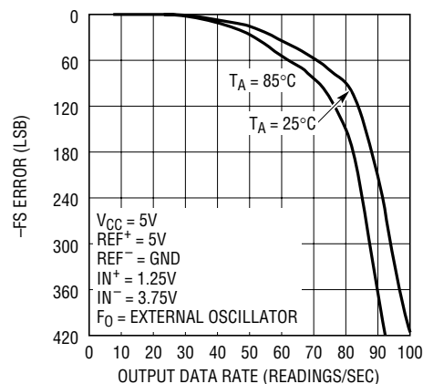
Figure 26. -FS Error vs Output Data Rate and Temperature
