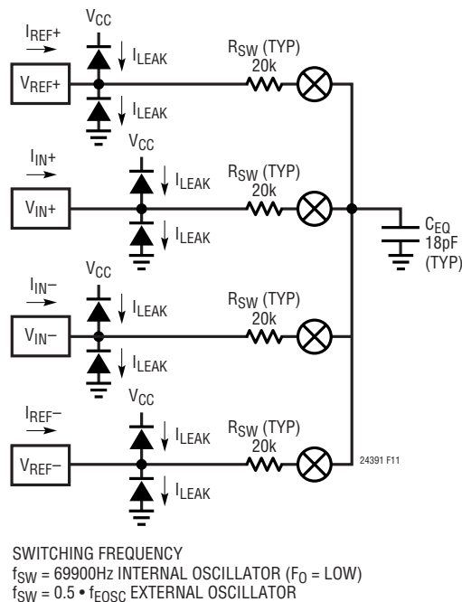
Figure 12. LTC2439-1 Equivalent Analog Input Circuit
