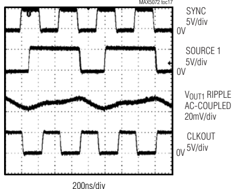
EXTERNAL SYNCHRONIZATION
