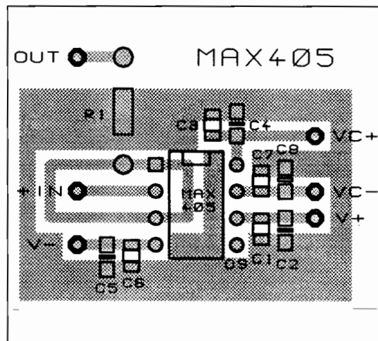
Figure 4. Typical Board Layout (see Typical Application Circuit)
