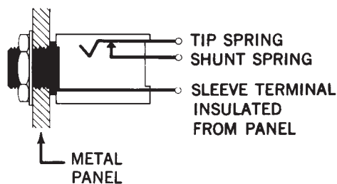
INSULATED MOUNTING
