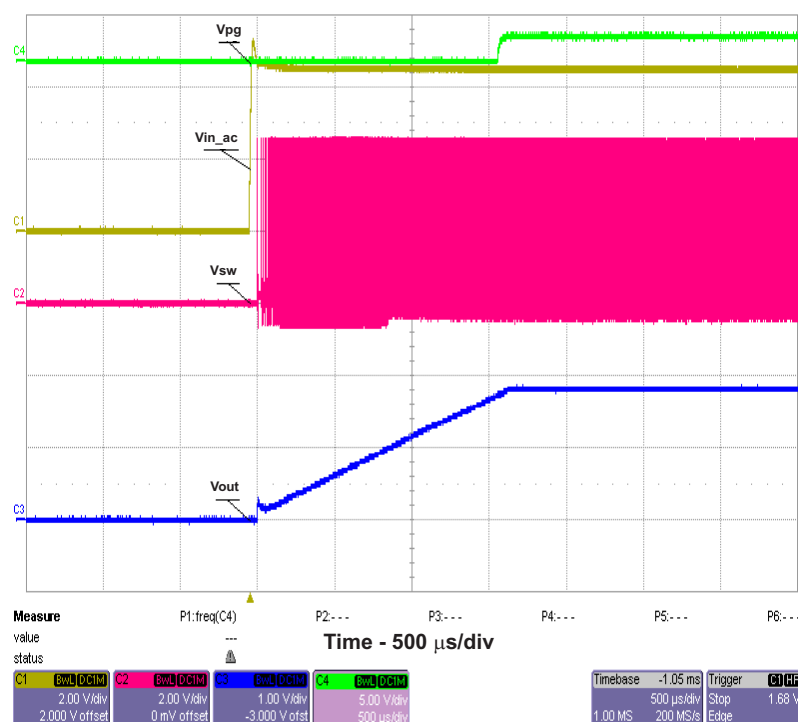
Figure 6. Power Up by Hot Plugging Vin
