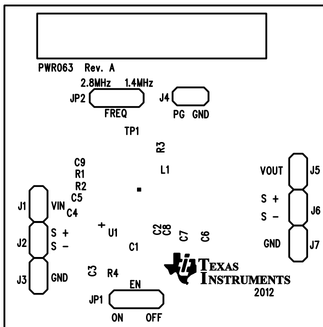
Figure 9. Assembly Layer
