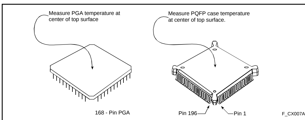
Figure 5. Measuring 80960CA PGA and PQFP Case Temperature
