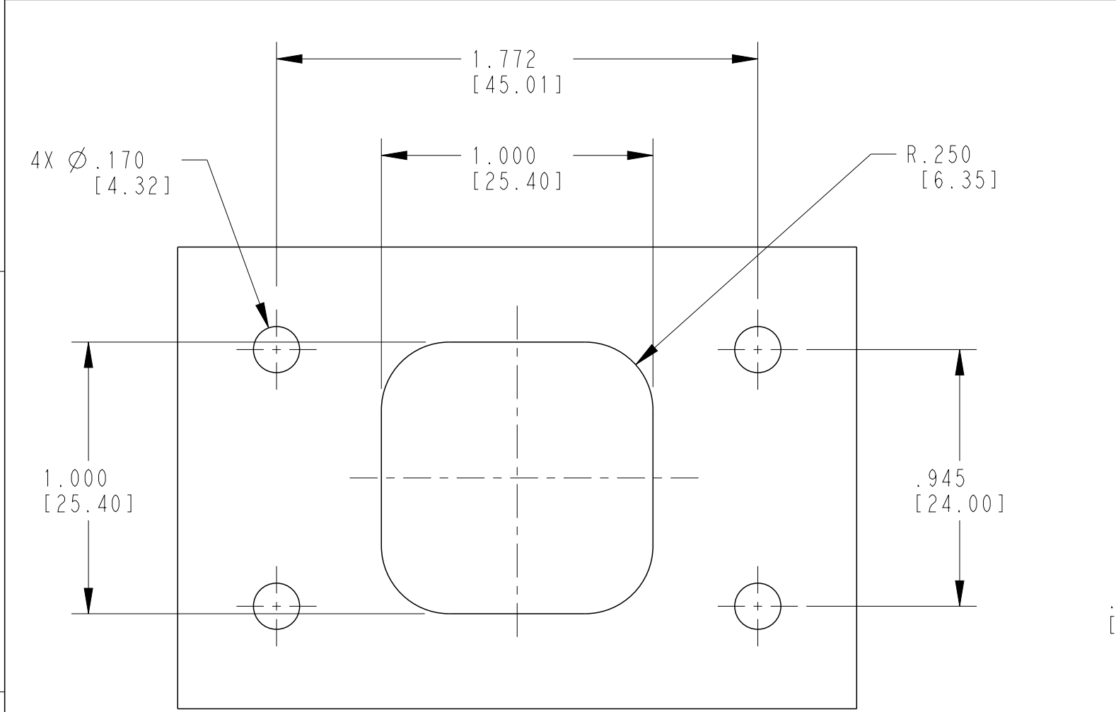
RECOMMENDED CUTOUT FRONT AND REAR MOUNT
