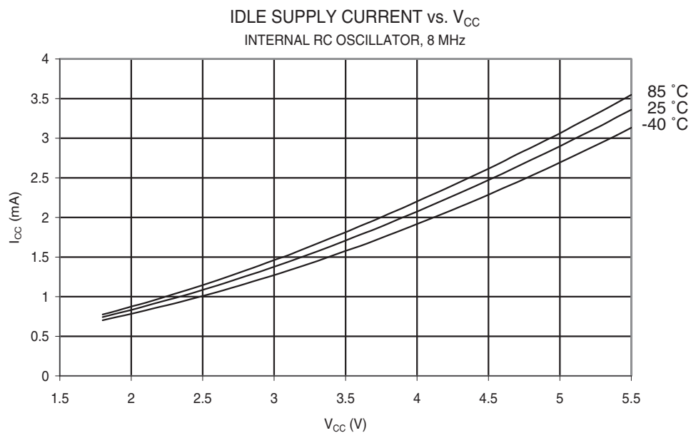
Figure 139. Idle Supply Current vs. V_{CC} (Internal RC Oscillator, 8 MHz)
