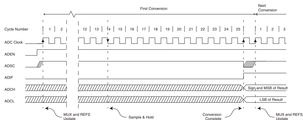
Figure 86. ADC Timing Diagram, First Conversion (Single Conversion Mode)
