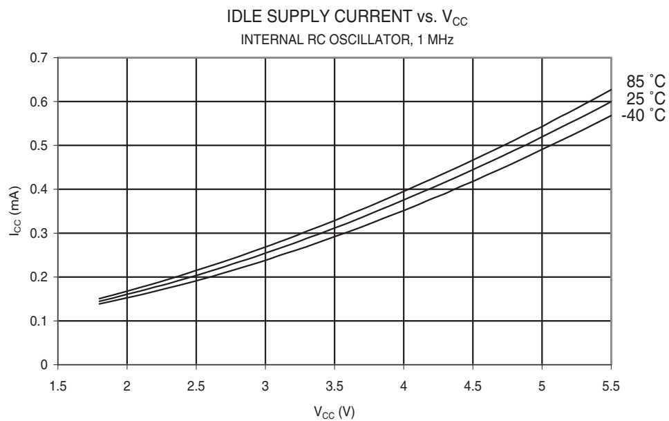
Figure 140. Idle Supply Current vs. V_{CC} (Internal RC Oscillator, 1 MHz)
