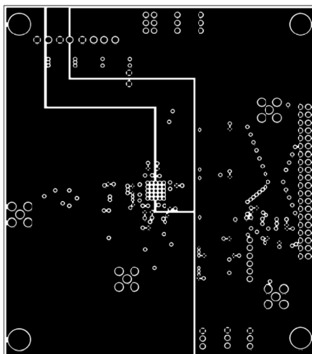
Figure 19. Power Plane
