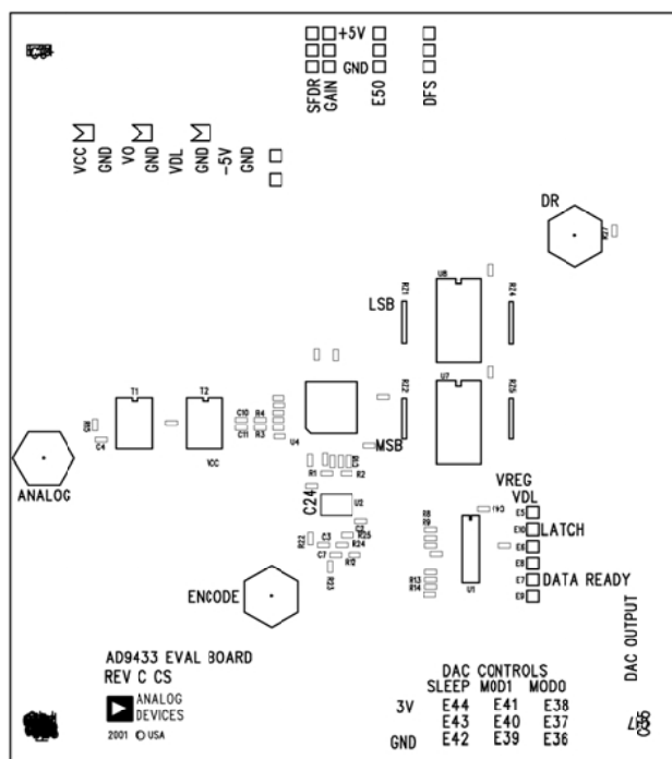
Figure 16. Top Silkscreen
