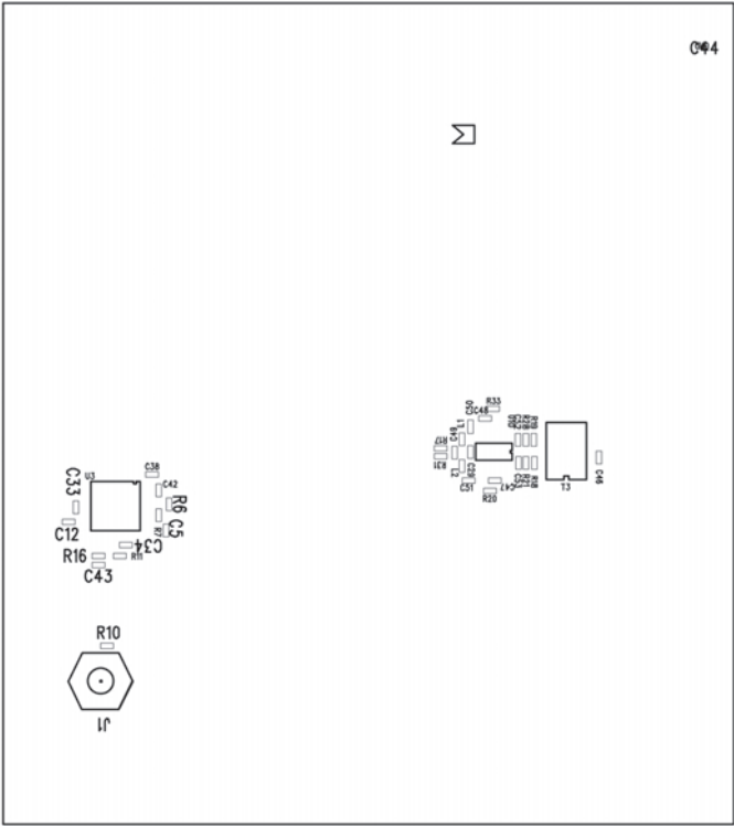
Figure 21. Bottom Silkscreen
