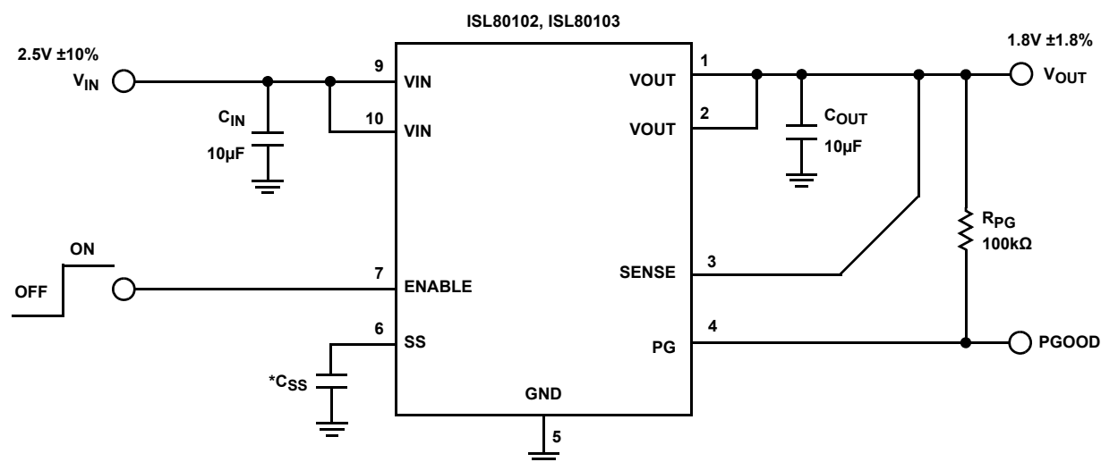
FIGURE 1. TYPICAL APPLICATION
