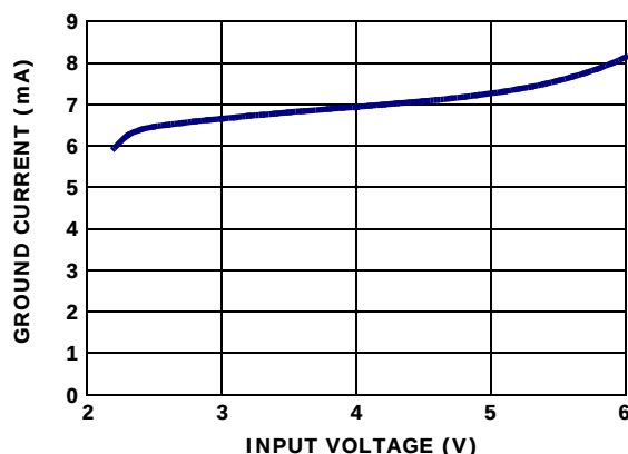
FIGURE 6. GROUND CURRENT vs SUPPLY VOLTAGE
