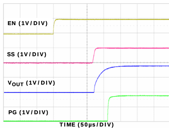
FIGURE 16. ENABLE START-UP
