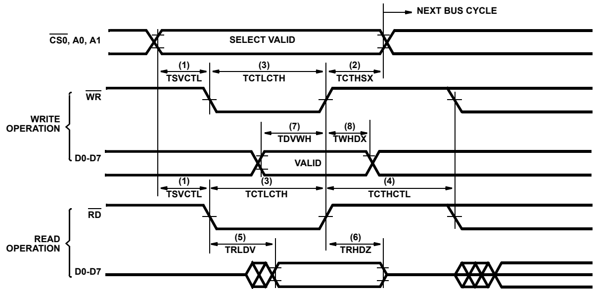
FIGURE 14. BUS OPERATION
