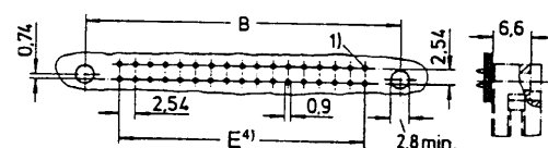
PC. board layout
