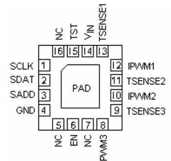
Top View : TQFN 16-Lead 3 x 3 mm 2
