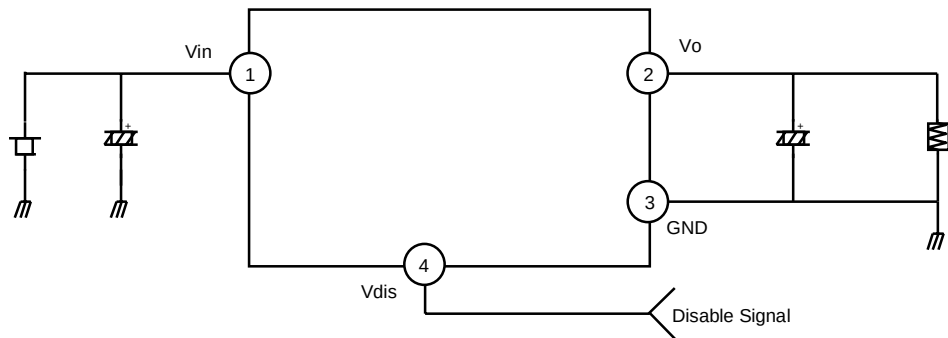
FIG.1 APPLICATION CIRCUIT
