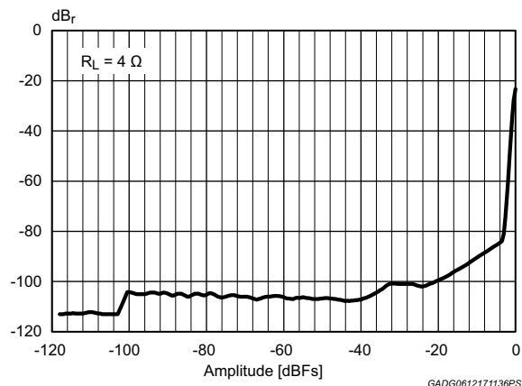
Figure 36. Dynamic range
