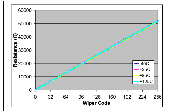
FIGURE 2-42: 50 kΩ – R_{WB} (Ω) vs. Wiper Setting and Ambient Temperature ( V_{DD} = 5.5\text{V} , I_W = 90\text{ }\mu\text{A} ).
