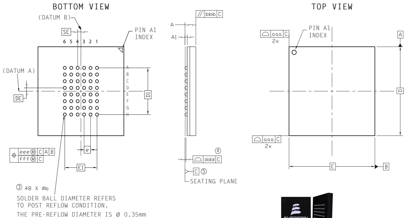
Figure 5.1 48-FBGA
