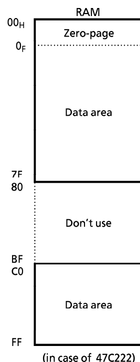
Figure 1-2. RAM addressing
