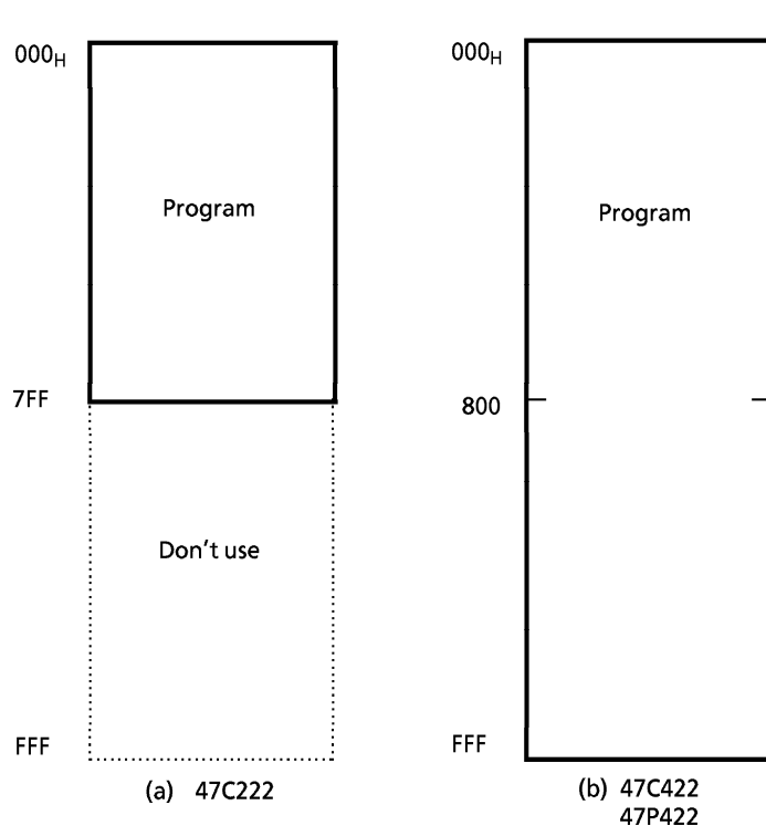
Figure 1-1. Program area (ROM)
