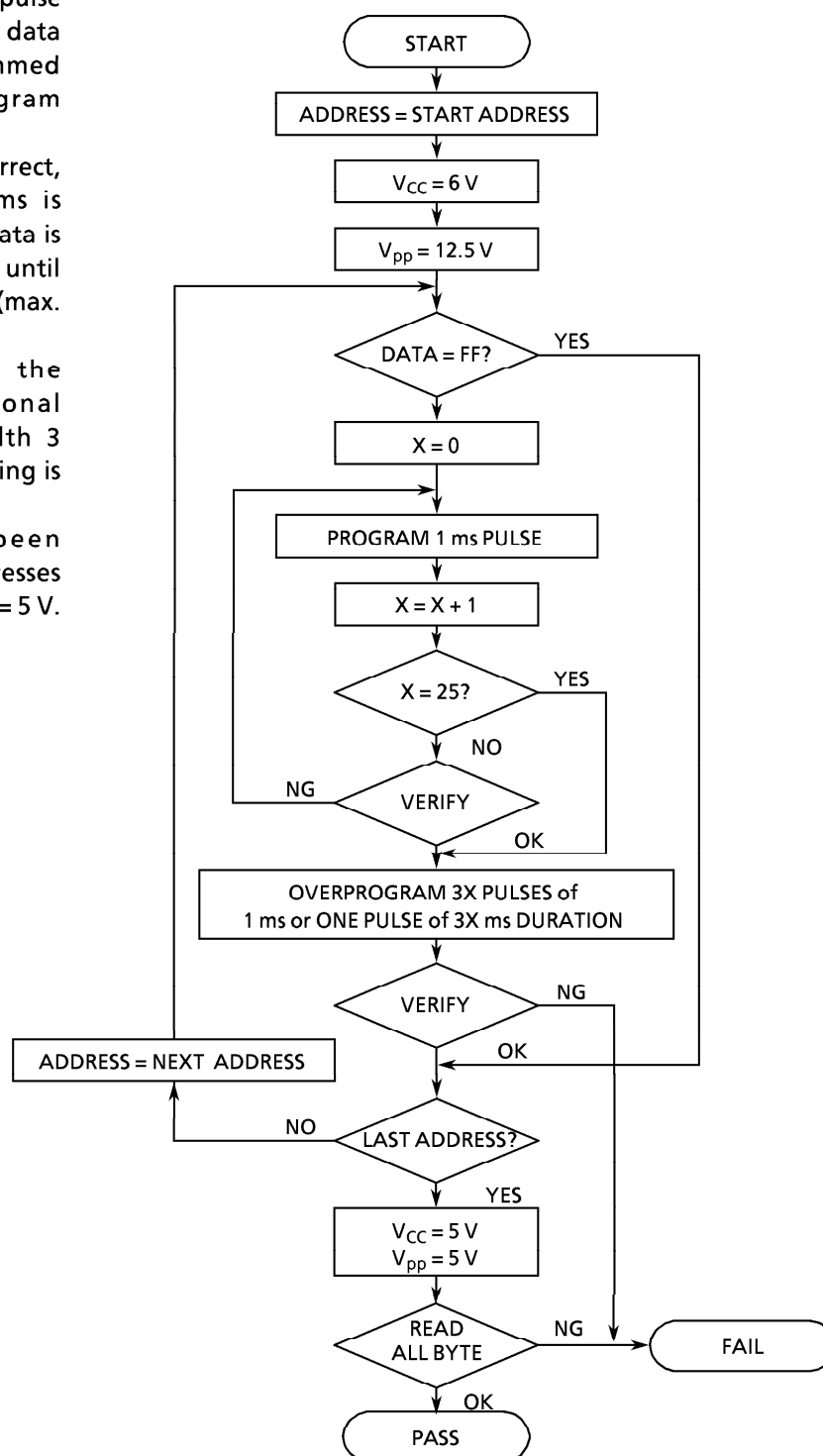
Figure 1-6. Flow Chart
