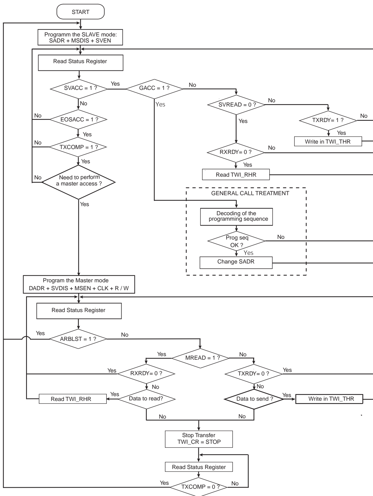
Figure 29-23. Multi-master Flowchart
