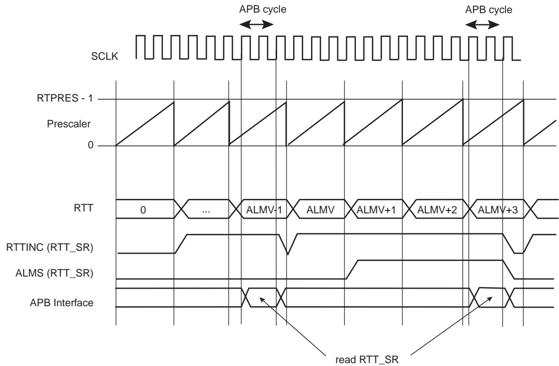
Figure 14-2. RTT Counting
