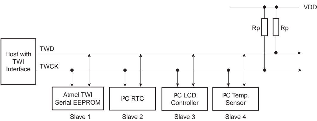
Figure 29-2. Application Block Diagram
