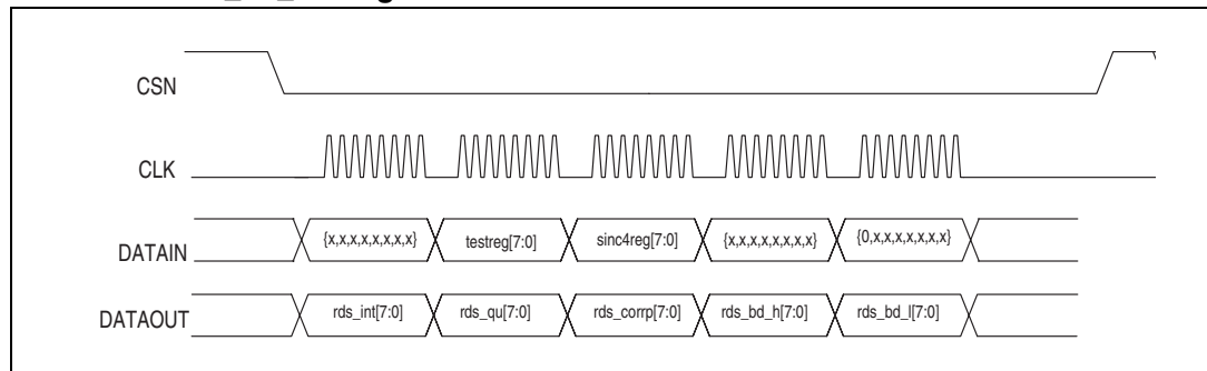
Figure 20. Read out RDS data and related flags, no update of rds_int and rds_bd_ctrl registers
