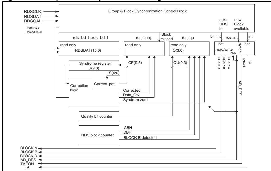
Figure 6. Group and block synchronization diagram
