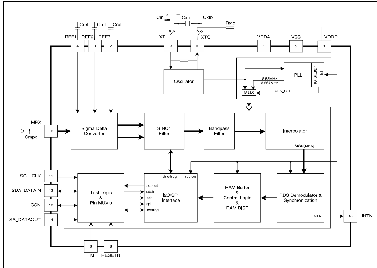
Figure 2. RDS decoder block diagram
