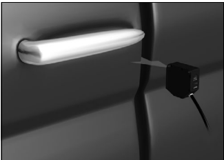
Door gap measurement
