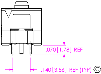
FIG 5 -RF1 OPTION (QFS-052-04.25-X-D-RF1 SHOWN) (SAME AS FIG 3, UNLESS OTHERWISE STATED) (NOT AVAILABLE WITH -A OR -GP OPTIONS) (AVAILABLE ON -04.25 LEAD STYLE, POSITIONS -026, -052, & -078 ONLY)
