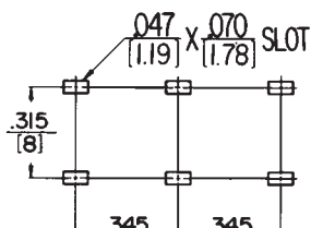
RECOMMENDED PC BOARD LAYOUT (Component Side)
