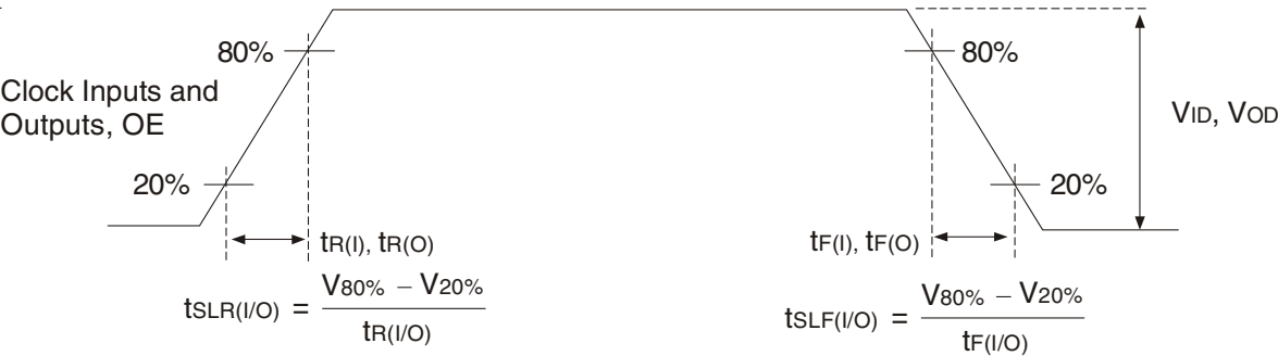
Input and Output Slew Rates
