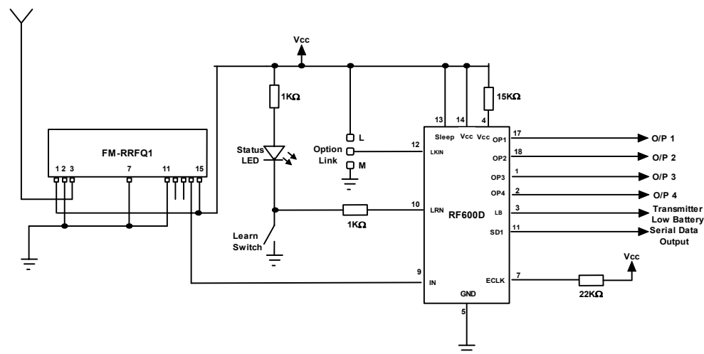
Receiver Circuit
