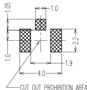
RECOMMENDED PCB PATTERN
