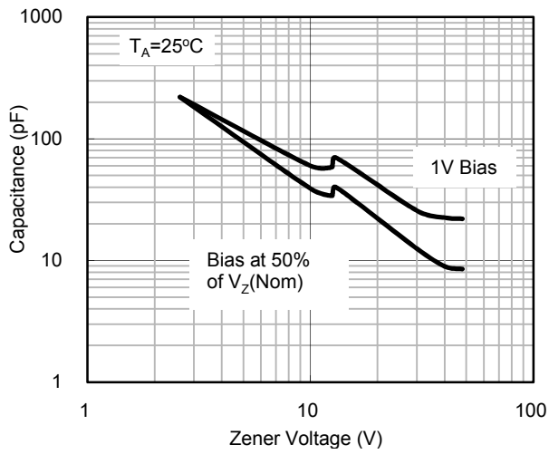
Fig.5 Typical Capacitance
