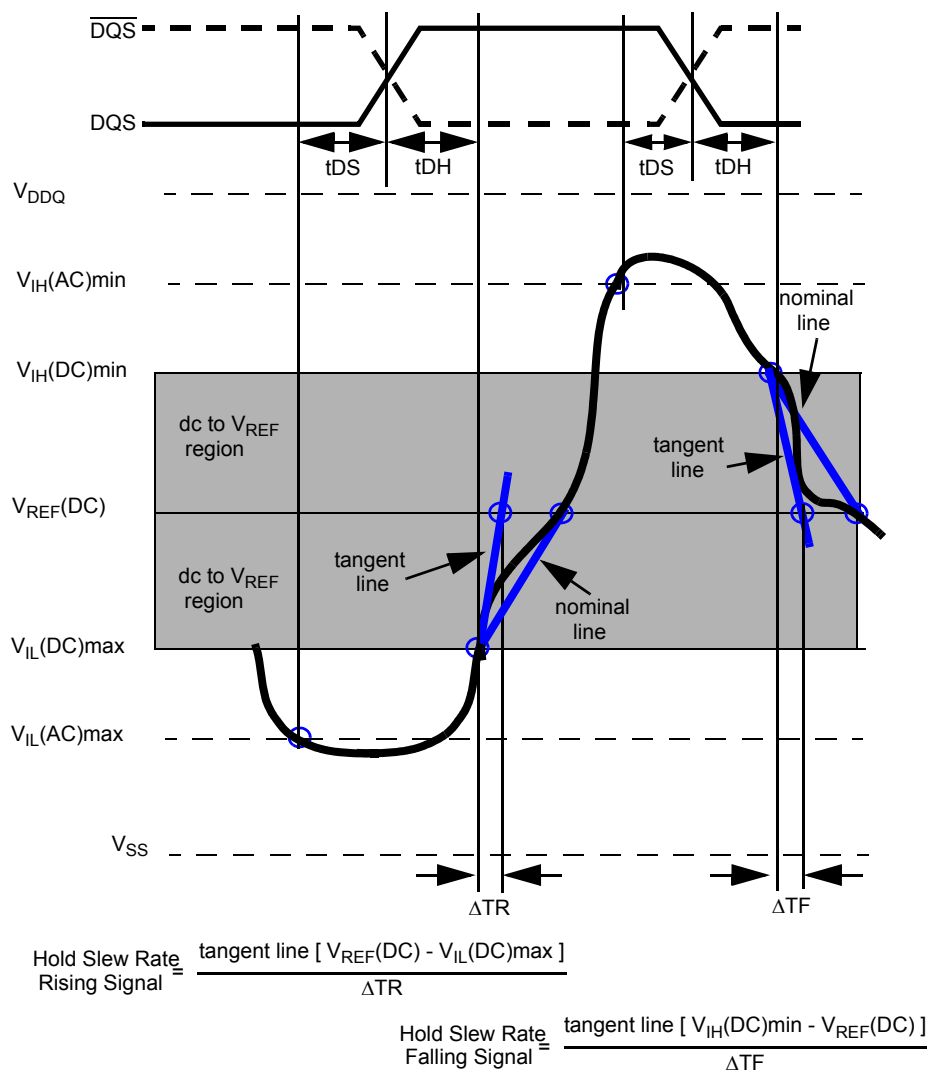
Figure 13. Illustration of tangent line for tDH (differential DQS, \overline{\text{DQS}} )
