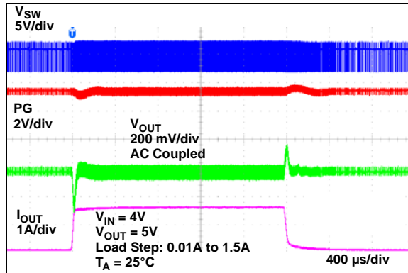
FIGURE 2-13: Load Transient ( V_{IN} = 4\text{V} ), Adjustable Output Version.
