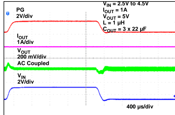
FIGURE 2-16: Line Transient ( V_{IN} = 2.5\text{V} to 4.5\text{V} ), Adjustable Output Version.
