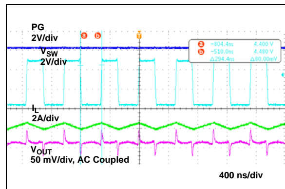
FIGURE 2-17: Switching Waveforms ( V_{IN} = 2.5\text{V} , V_{OUT} = 5\text{V} , I_{OUT} = 1.5\text{A} ), Adjustable Output Version.
