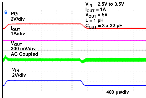
FIGURE 2-15: Line Transient ( V_{IN} = 2.5\text{V} to 3.5\text{V} ), Adjustable Output Version.
