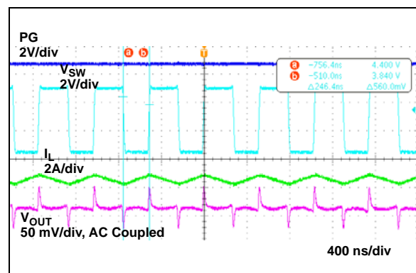
FIGURE 2-18: Switching Waveforms ( V_{IN} = 3\text{V} , V_{OUT} = 5\text{V} , I_{OUT} = 2\text{A} ), Adjustable Output Version.
