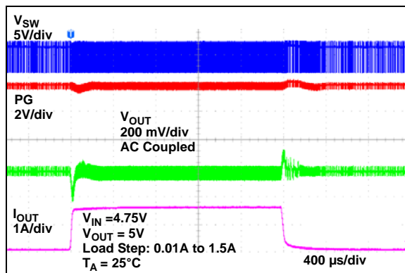
FIGURE 2-14: Load Transient ( V_{IN} = 4.75\text{V} ), Adjustable Output Version.
