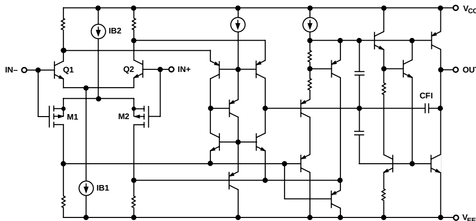
Figure 27. Simplified Schematic
