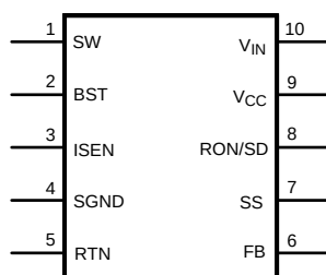
10-Lead WSON
