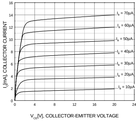
Figure 1. Static Characteristics
