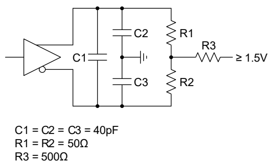
Figure 6. Tri-State High Load Circuit
