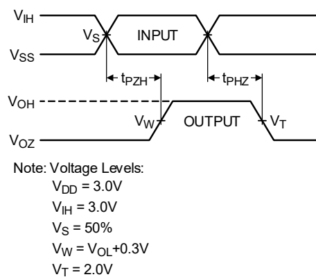
Figure 7. Tri-State High Timing Diagram
