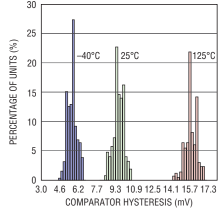
Hysteresis Distribution
