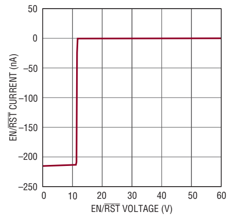
EN/RST Current vs Voltage
