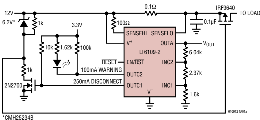
Circuit Fault Protection with Latching Load Disconnect and Early Warning Indication
