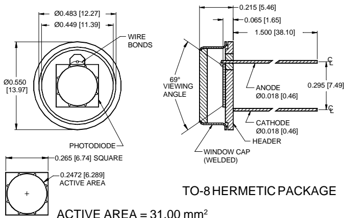
PACKAGE DIMENSIONS INCH [mm]
