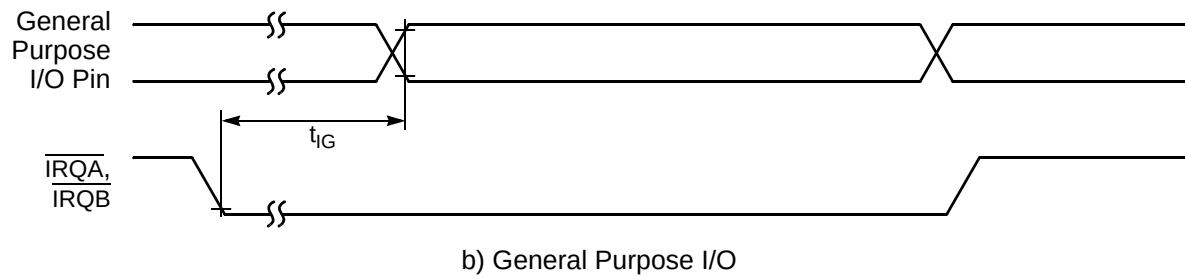
Figure 10-8 External Level-Sensitive Interrupt Timing
