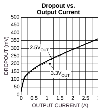
Adjustable Regulator
