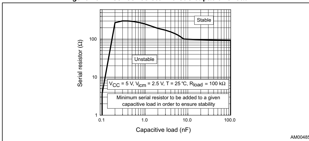
Figure 29. In series resistor versus capacitive load
