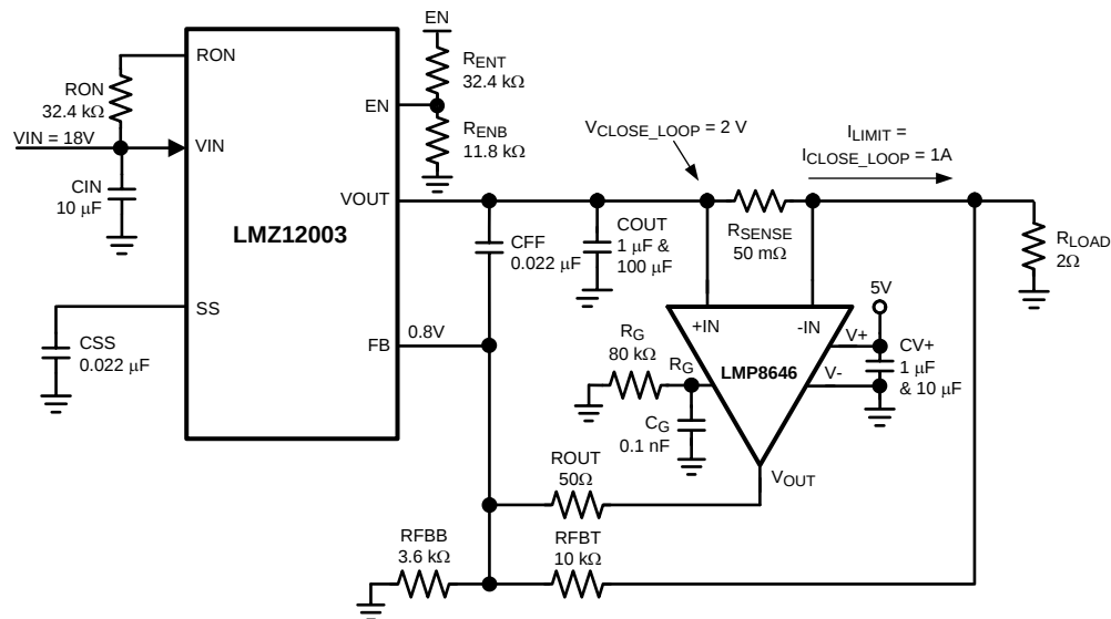
Figure 30. Resistive Load Application With LMZ12003 Regulator
