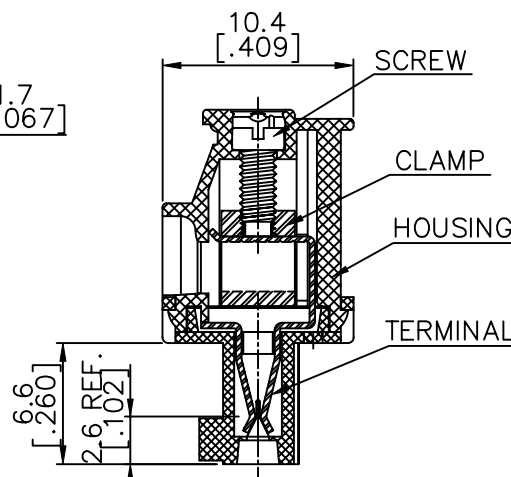
SECTION P-P
