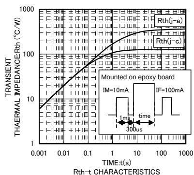
Rth-t CHARACTERISTICS
