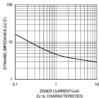
Zz-Iz CHARACTERISTICS
