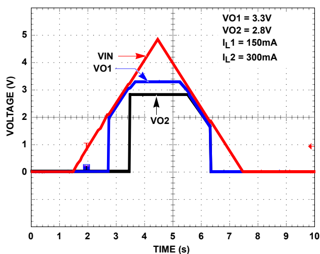
FIGURE 12. POWER-UP/POWER-DOWN
