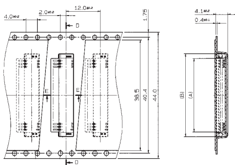
SECT. D-D
