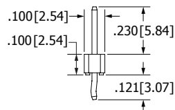
RETENTION LEAD MOUNTING (EXAMPLE P/N: AMC36SAAR)
