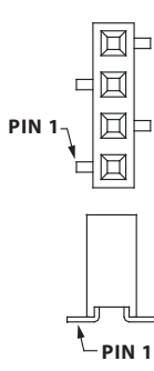
Single Row SMT, Pin 1 Left (C)
