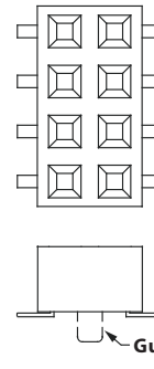
Dual Row SMT, With Guide Posts (P)
