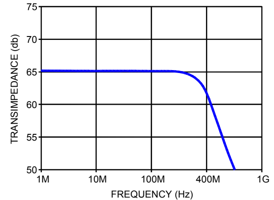
Fig. 6: TOTAL FREQUENCY RESPONSE
