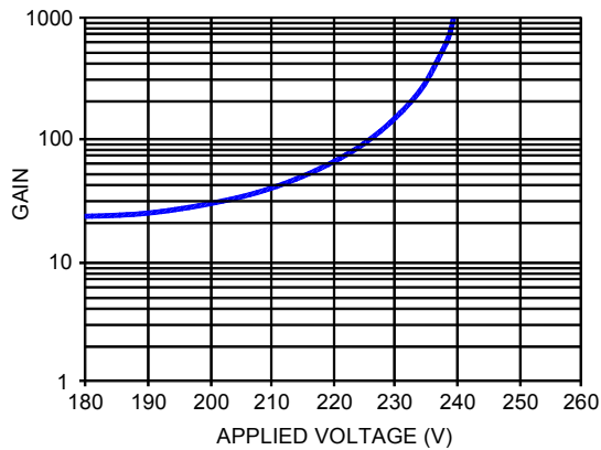
Fig. 1: APD GAIN vs BIAS VOLTAGE
