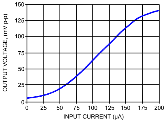
Fig. 5: AMPLIFIER TRANSFER FUNCTION
