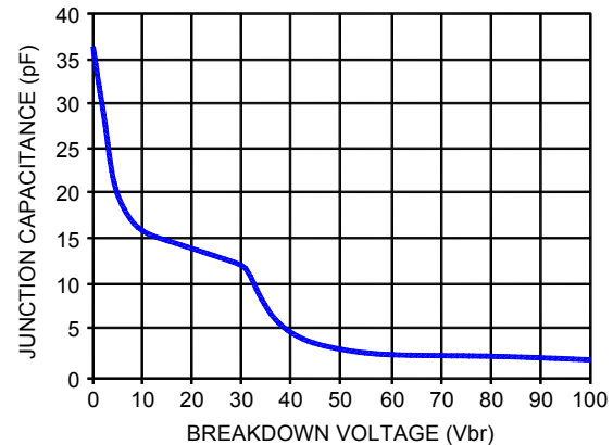
Fig.4 : APD CAPACITANCE vs VOLTAGE
