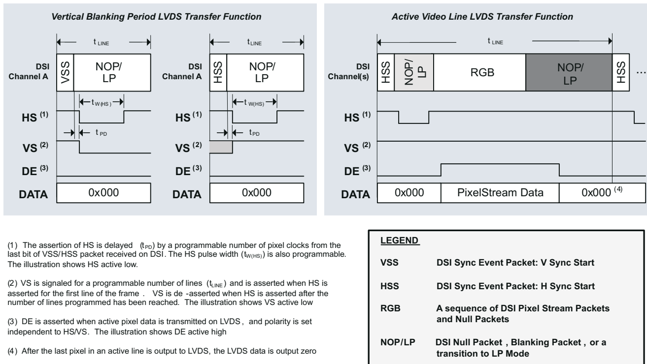
Figure 7-12. DSI Channel Transmission and Transfer Function
