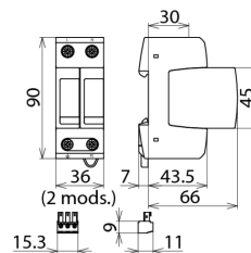
Dimension drawing DG M TT 2P ... FM
