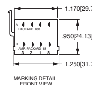
VCH CONNECTOR HOUSING
